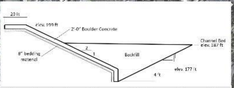
Cross-Section View of Proposed Pre-Formed Scour Hole
